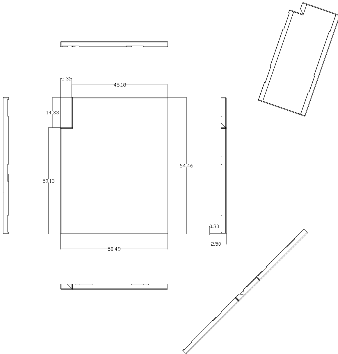
Shielding cover drawing
